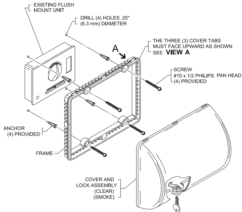
FLUSH MOUNT
