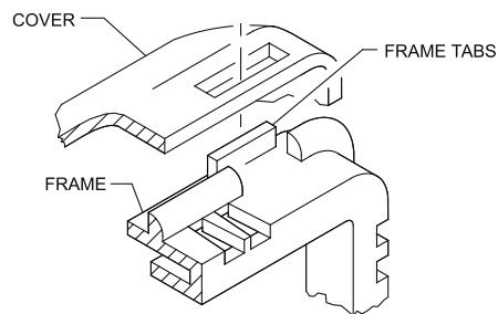
VIEW A
